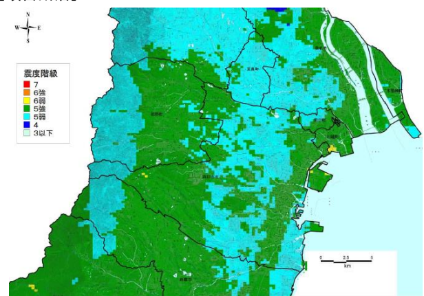
[頓宮断層]
